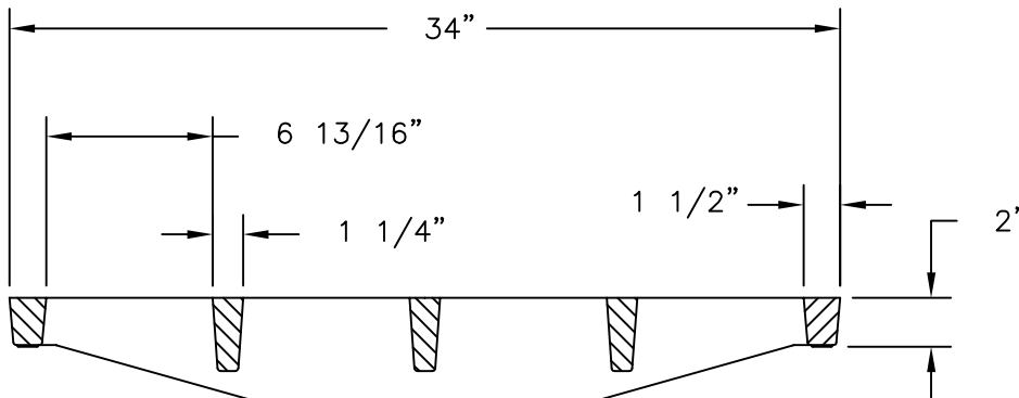
GRATE SECTION
